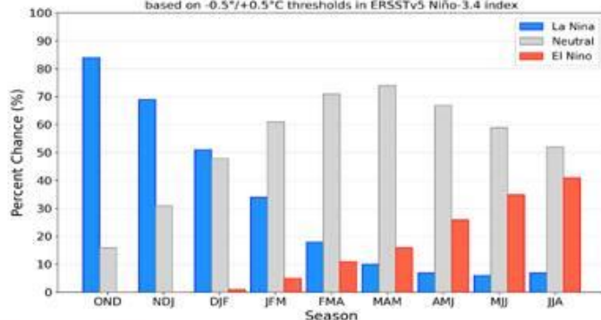
Official NOAA CPC ENSO Probabilities (issued November 2025) based on -0.5^{\circ}/+0.5^{\circ}\text{C} thresholds in ERSSTv5 Niño-3.4 index
